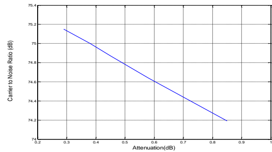
Fig.5 Attenuation and Carrier to Noise Ratio (dB)
