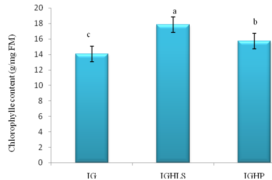
Fig.4 The chlorophyll content in different experimental greenhouses, (IG) Insulated greenhouse as a reference, (IGHLS): Insulated greenhouse equipped with a solar air collector and IGHP which is insulated greenhouse heated via a heat pump.
