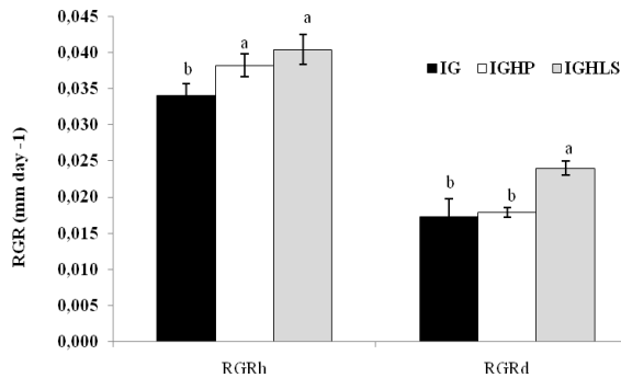
Fig.5 The Relative Growth Rate (RGR) of height and diameter stem of ten plants in experimental greenhouses.
