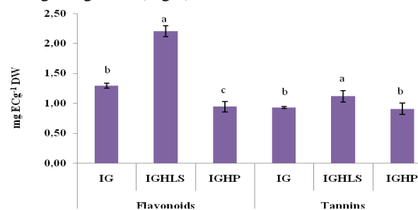
Fig.8 Effects of microclimatic conditions on flavonoids and tannins in tomatoes of IG, IGHP and IGHLS. (IG) Insulated greenhouse as a reference, (IGHLS): Insulated greenhouse equipped with a solar air collector and IGHP which is insulated greenhouse heated via a heat pump.
