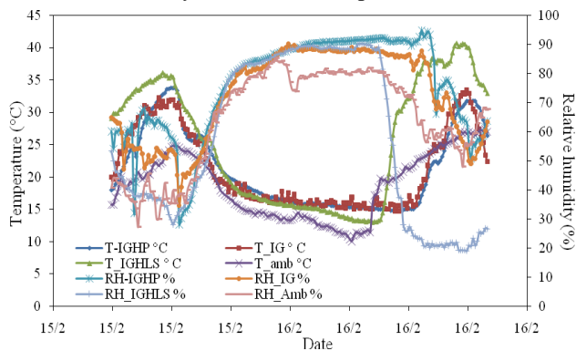
Fig.3 Ambient air temperature and relative humidity and inside the experimental greenhouses as a function of days (15th-16th February, 2014).
