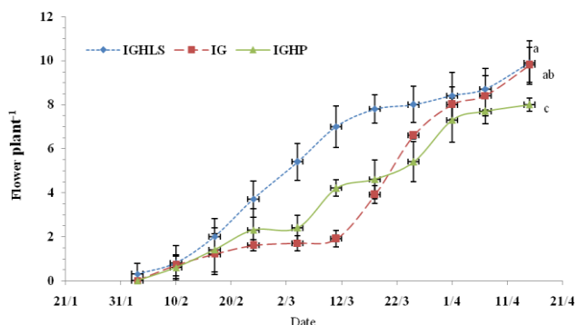
Fig.6 The average flower number plant -1 in (IG): Insulated greenhouse, (IGHLS): Insulated greenhouse equipped with a solar air collector and IGHP: insulated greenhouse heated via heat pump.
