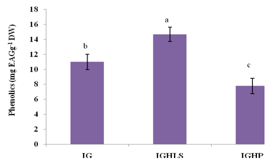
Fig.7 Effects of microclimatic conditions on phenolics in tomatoes of (IG): Insulated greenhouse, (IGHLS): Insulated greenhouse equipped with a solar air collector and IGHP: insulated greenhouse heated via heat pump.
