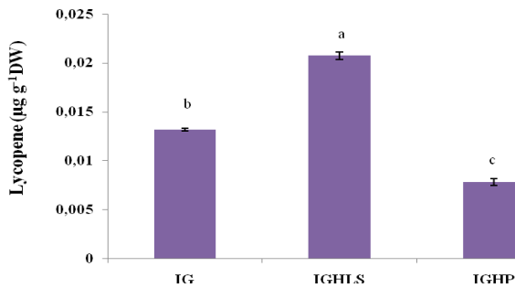
Fig.9 Effects of microclimatic conditions on lycopene in tomatoes of IG, IGHLS and IGHP. (IG) Insulated greenhouse as a reference, (IGHLS): Insulated greenhouse equipped with a solar air collector and IGHP which is insulated greenhouse heated via a heat pump.
