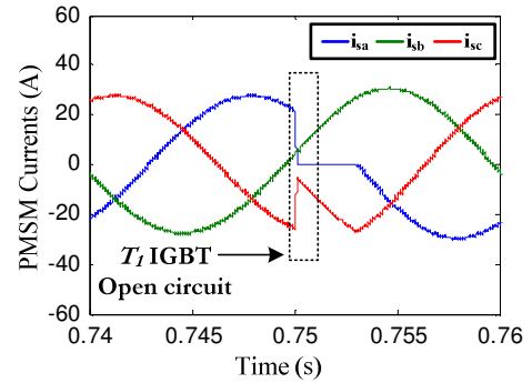
Fig. 5. The impact of the T_1 IGBT open-circuit on the stator currents i_{sa} , i_{sb} and i_{sc} under 10% rated load torque and 600 rpm operating conditions.
