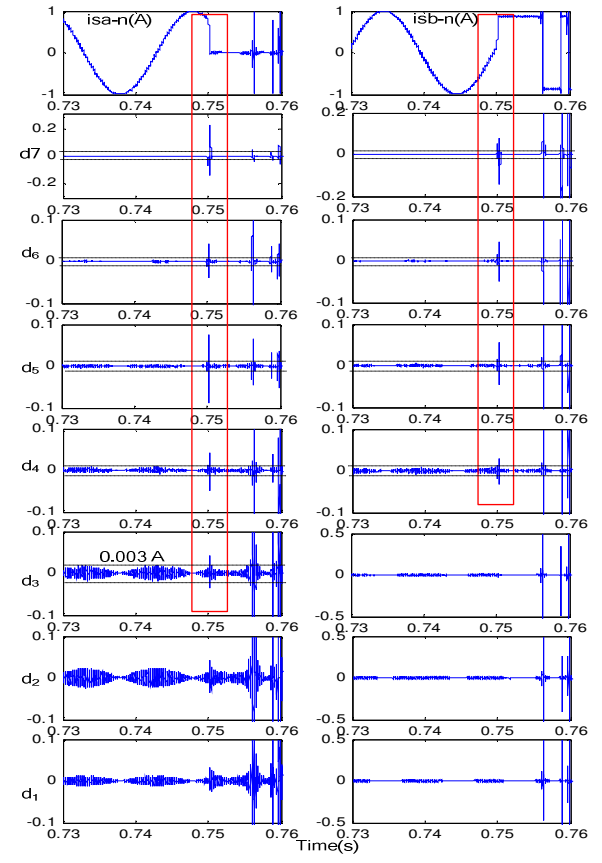
Fig. 9. Single open phase fault detection using stator currents i_{sa-n} and i_{sb-n} MRA
