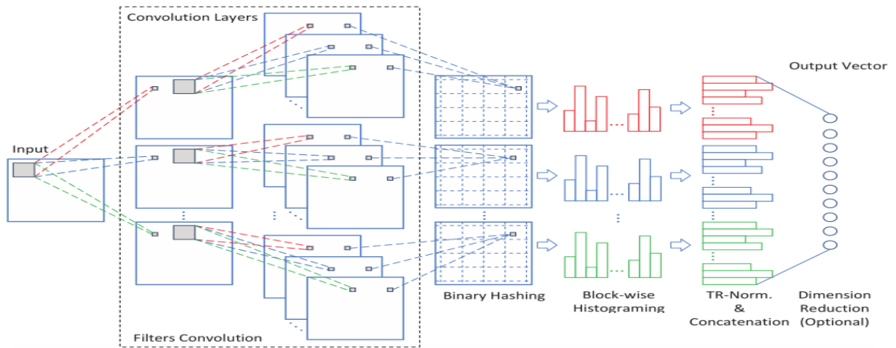
Fig. 2. The block diagram of the proposed DCTNet [10].
