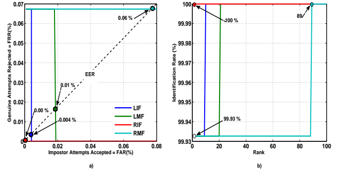
Fig. 6. Unimodal system results a) ROC curves b) CMC curves.
