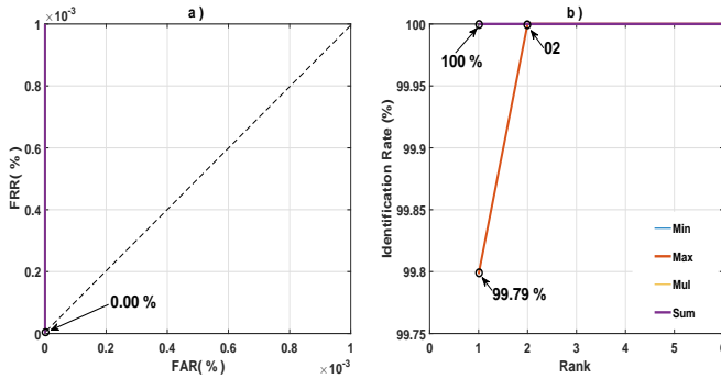
Fig. 8. Multimodal system results a) ROC curves b) CMC curves.
