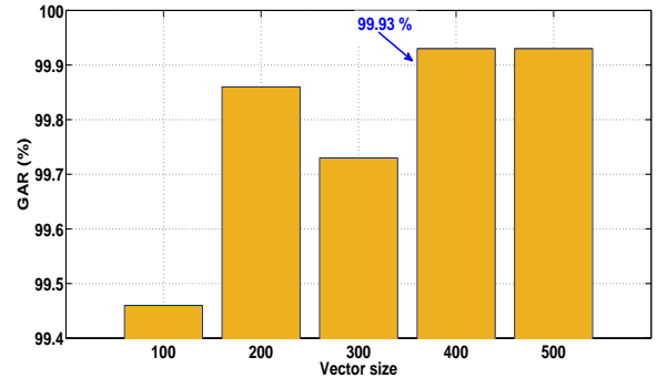
Fig. 5. DCTNet parameter adaptation the GAR against vector size.
