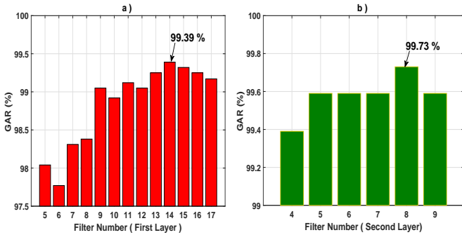
Fig. 3. DCTNet parameter adaptation a) GAR against Filter number in first layer, b) GAR against Filter number in second layer.
